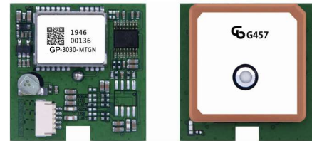
Figure : GP -3030- MTGN Top View
